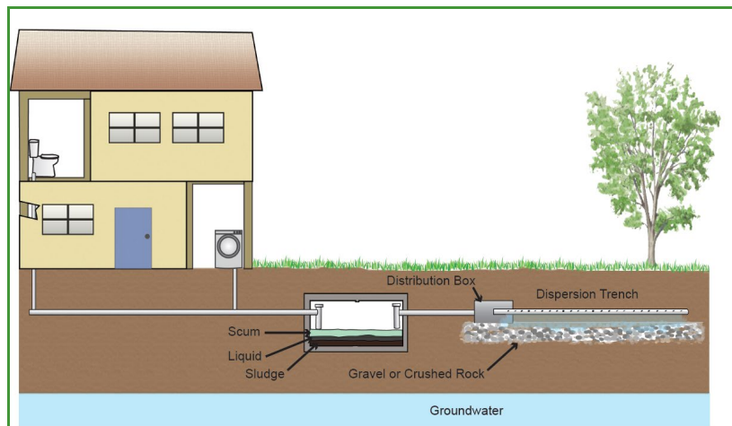
Components of a standard septic system that would be inspected during a detailed system inspection.
